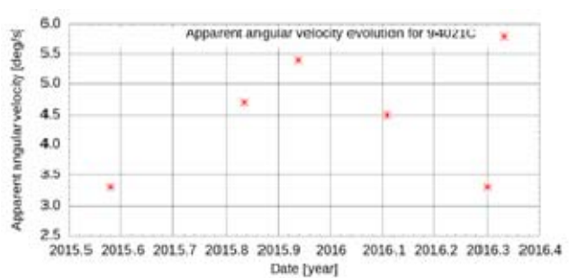
Fig. 10. One year evolution of the apparent angular velocity for GLONASS satellite 1994-021C from light curves acquired by ZIMLAT telescope between years 2015 and 2016.
