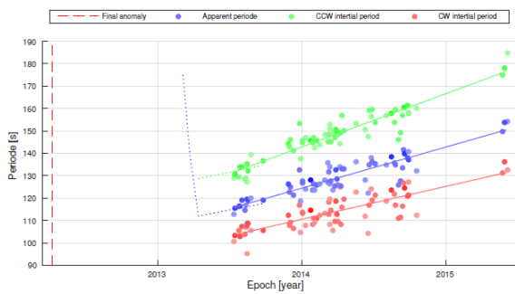
Fig. 7. Evolution of the synodic (blue) and the sidereal (red, green for clockwise and counterclockwise rotation) spin periods of Envisat as determined from SLR observations from Zimmerwald.
