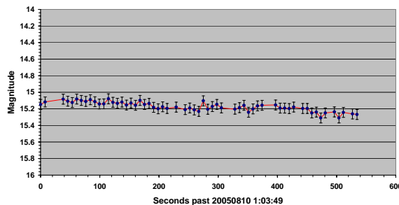
Fig. 15. Light curve of the object 'EGEO014' which has an area-to-mass ratio of 17 \text{ m}^2/\text{kg} .
