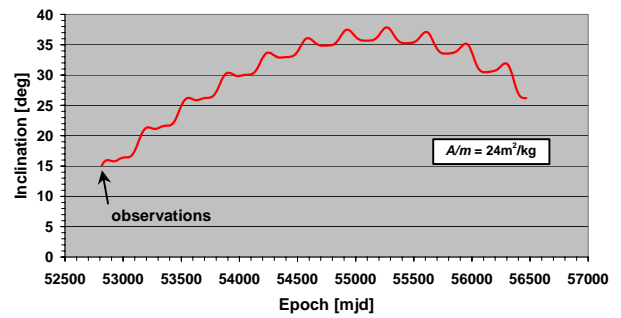
Fig. 12. Evolution of the inclination for an object of the new population over the next ten years.
