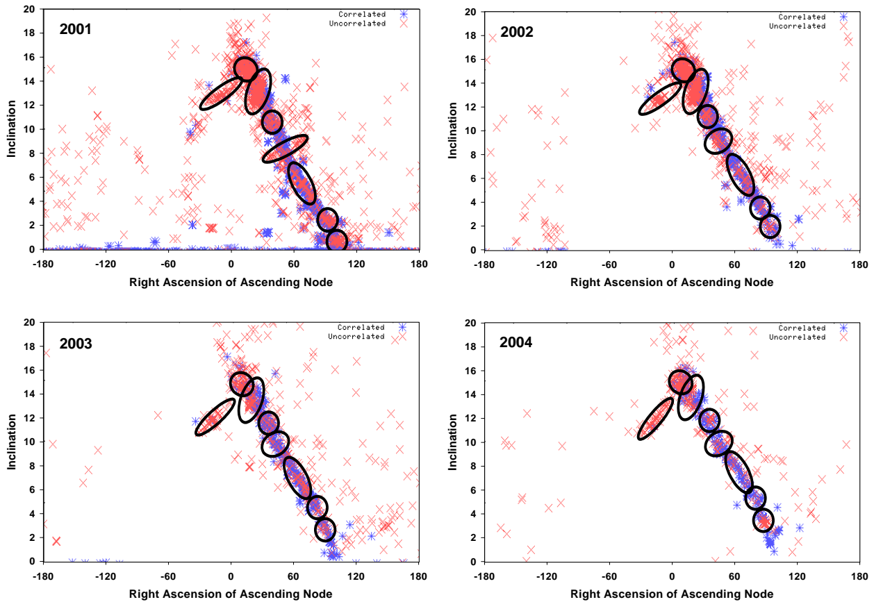
Fig. 4. Evolution of debris clouds (marked with circles) through the years 2001 to 2004 (uncorrelated detections are marked with crosses and correlated detections with asterisk respectively).
