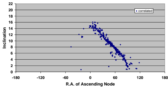
Fig. 2. Inclination i as a function of the right ascension of the ascending node \Omega for the correlated detections of the year 2004.
