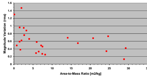
Fig. 13. Variation (rms) of the apparent magnitude as a function of the area-to-mass ratio for 28 uncorrelated objects of the new debris population.
