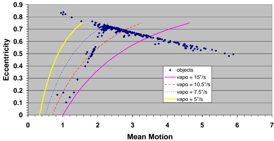
Fig. 9. Eccentricity as a function of the mean motion for the objects in the catalogue.
