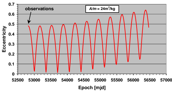
Fig. 11. Evolution of the eccentricity for an object of the new population over the next ten years.
