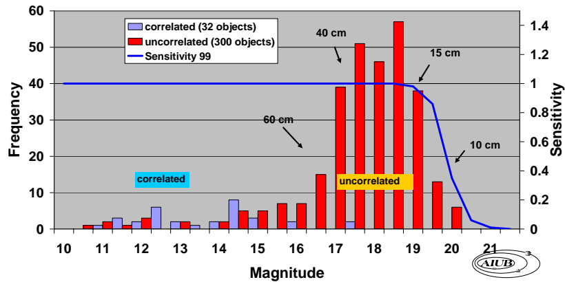
Fig. 5. Magnitude distribution for 332 objects with elliptical orbits.
