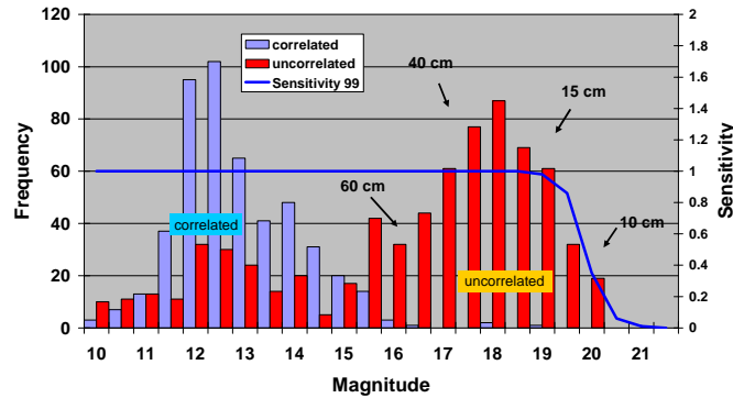
Fig. 1. Absolute magnitude distribution for the detections of the year 2004.
