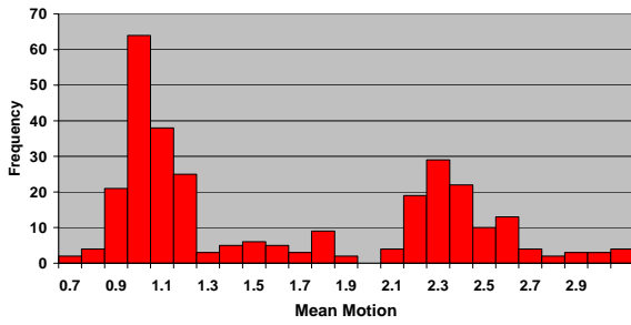
Fig. 6. Distribution of the mean motion for 332 objects with elliptical orbits. (Mean motion in rev. per day.)
