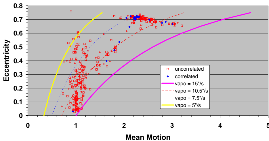
Fig. 8. Eccentricity as a function of the mean motion for 332 objects with elliptical orbits.
