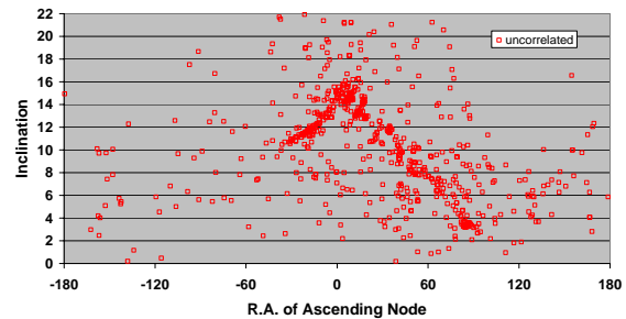
Fig. 3. Inclination i as a function of the right ascension of the ascending node \Omega for the uncorrelated detections of the year 2004.
