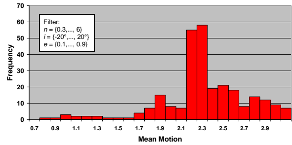
Fig. 7. Distribution of objects in the catalogue. (Mean motion in revolutions per day.)
