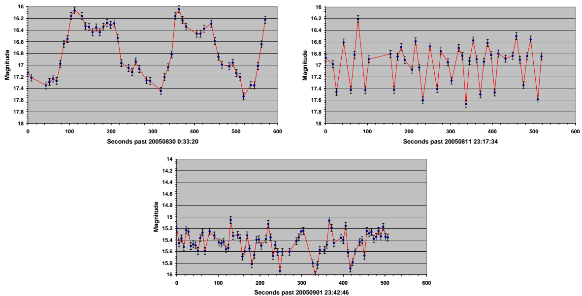
Fig. 14. Three light curves of the object 'EGEO021' which has an area-to-mass ratio of 4.6 m 2 /kg.
